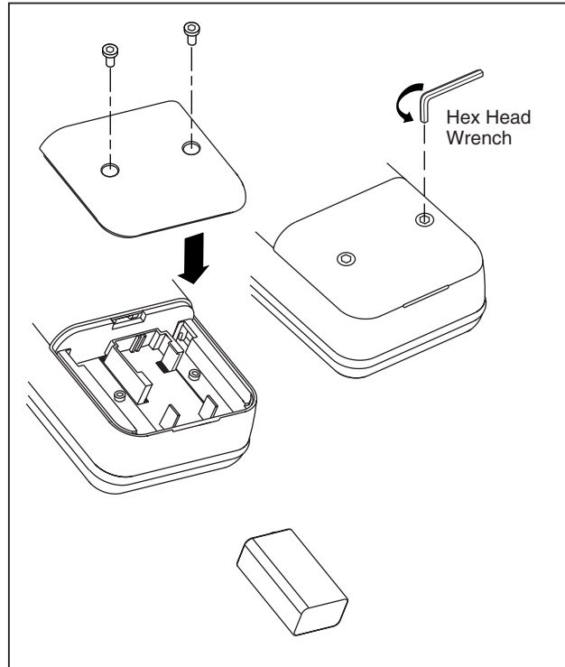
Figure 7. Battery Replacement
